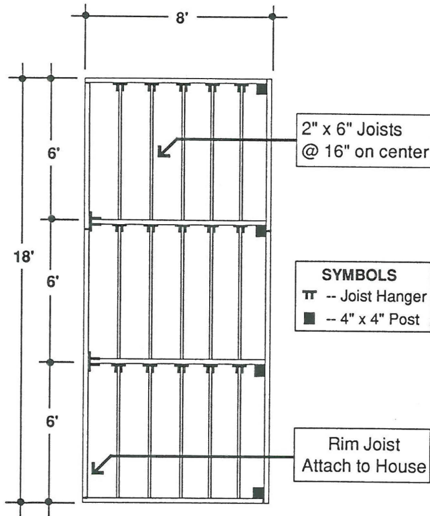
Deck Framing Layout
