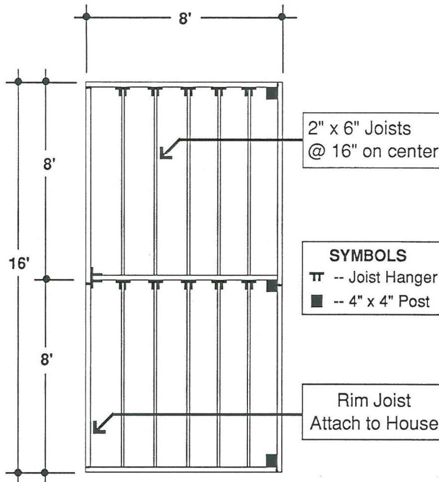
Deck Framing Layout
