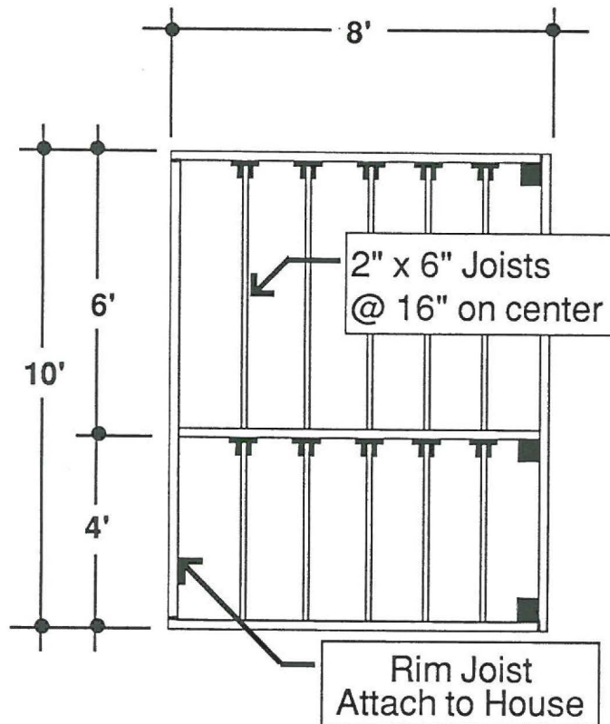
Deck Framing Layout
