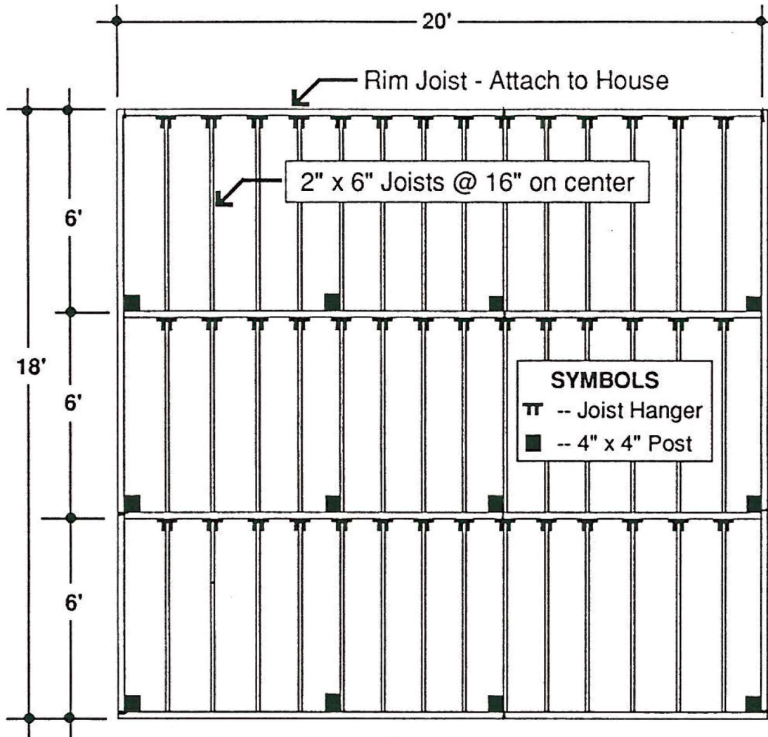
Deck Framing Layout
