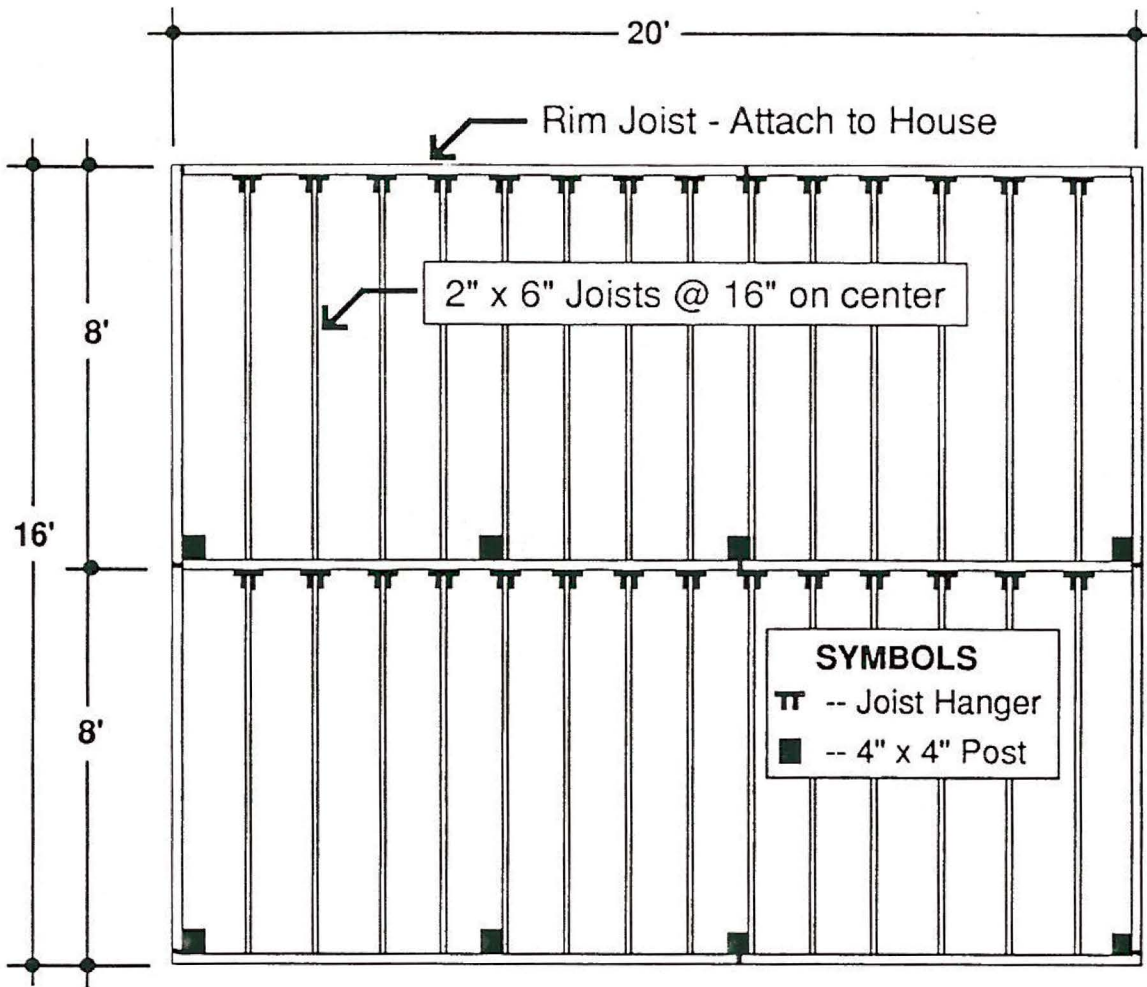
Deck Framing Layout
