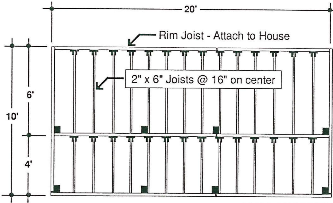
Deck Framing Layout
