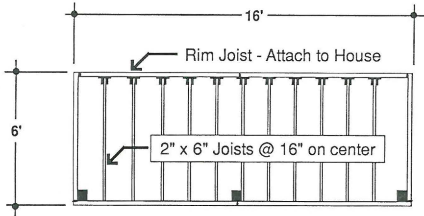
Deck Framing Layout
