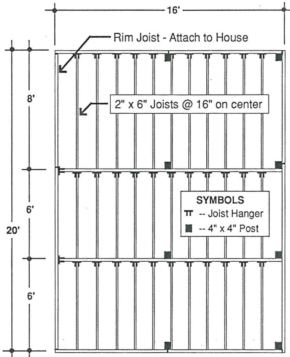
Deck Framing Layout
