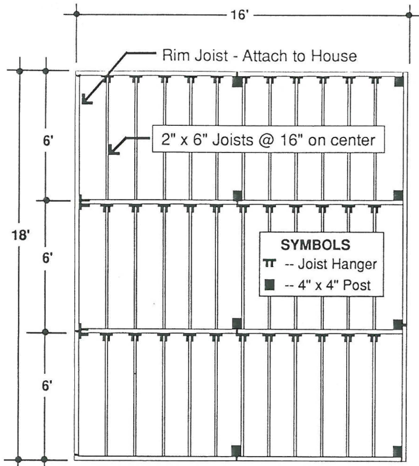
Deck Framing Layout
