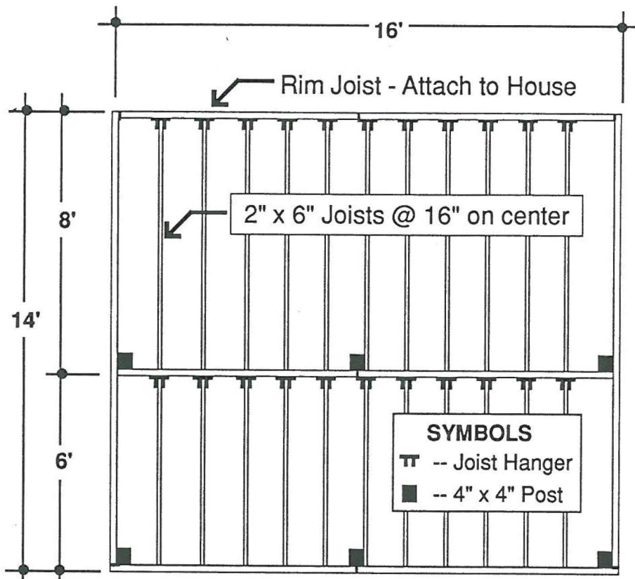
Deck Framing Layout
