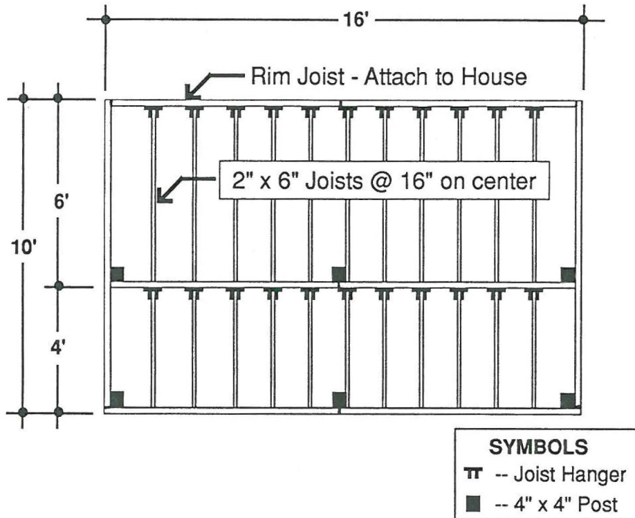
Deck Framing Layout
