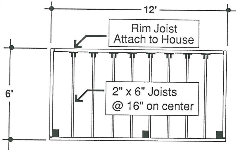
Deck Framing Layout
