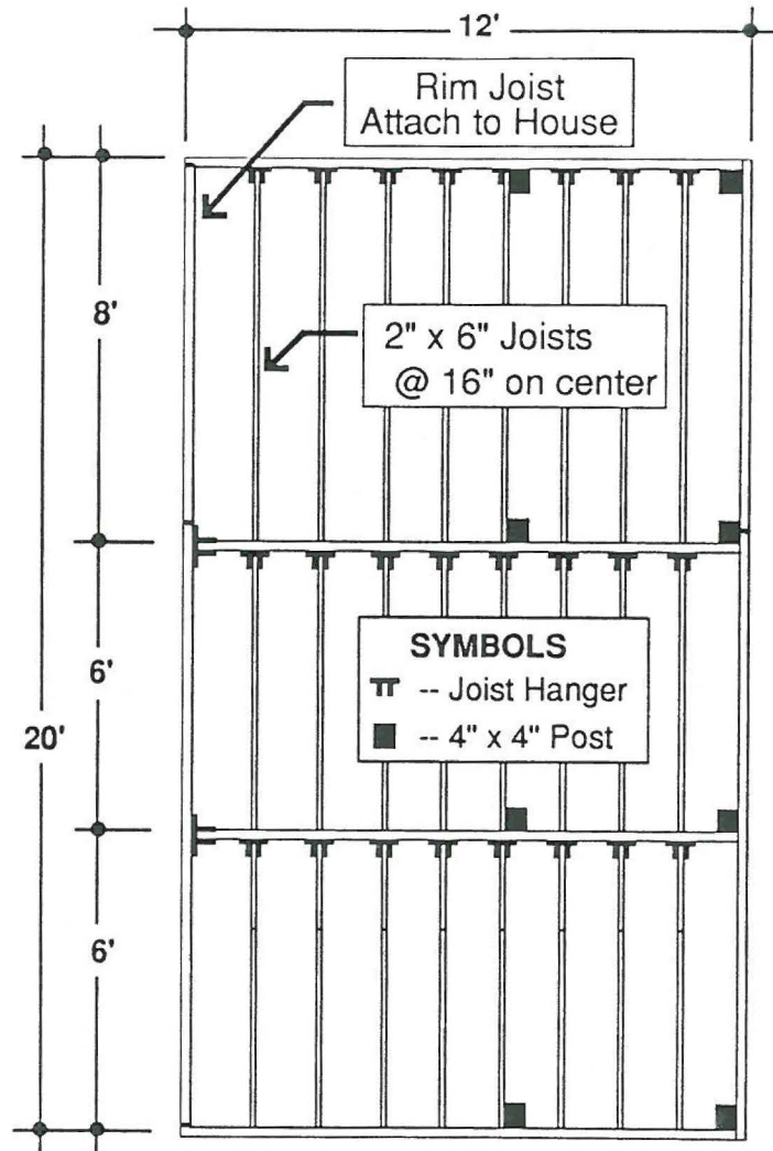
Deck Framing Layout
