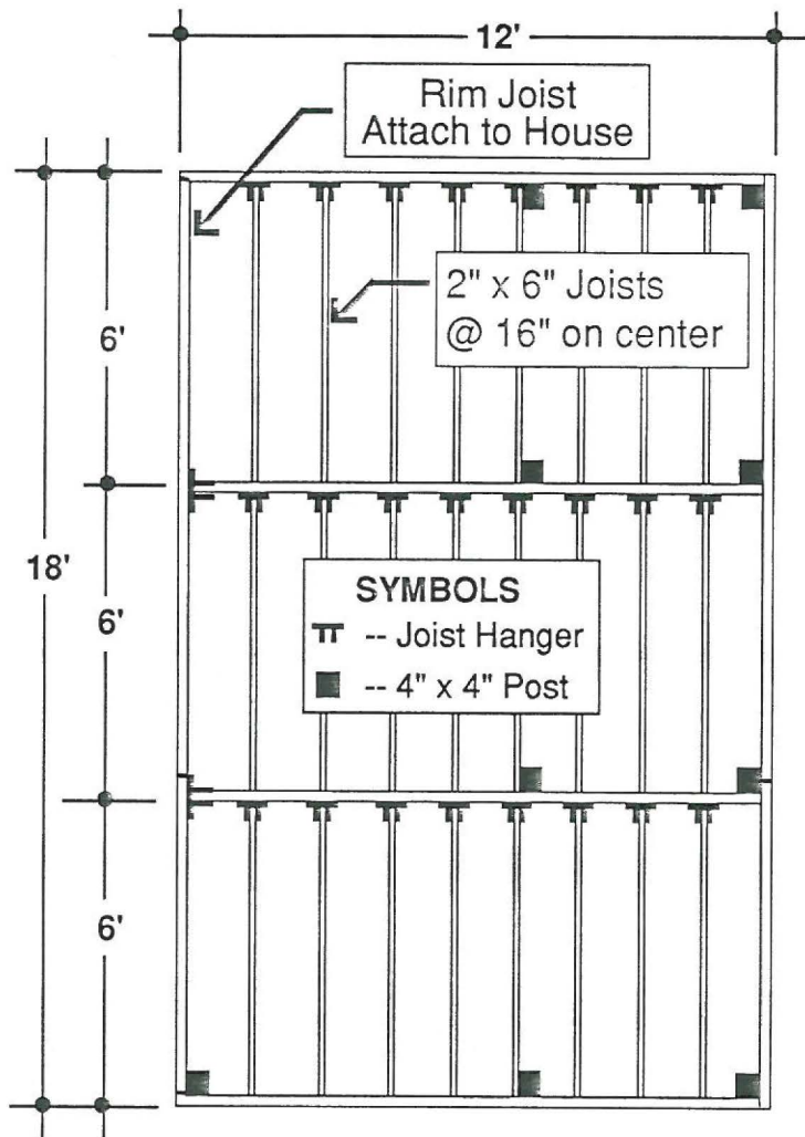
Deck Framing Layout
