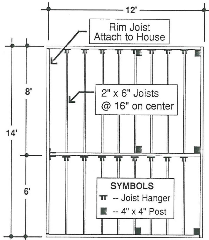
Deck Framing Layout
