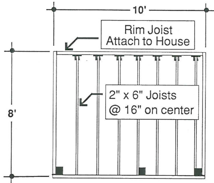
Deck Framing Layout
