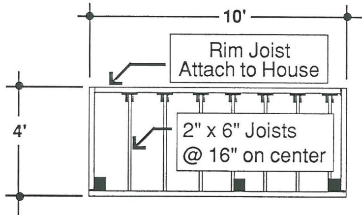
Deck Framing Layout
