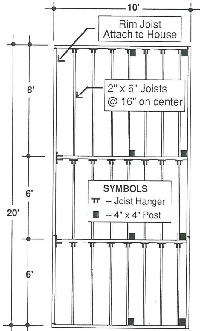
Deck Framing Layout
