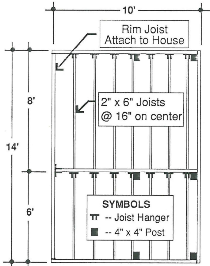
Deck Framing Layout
